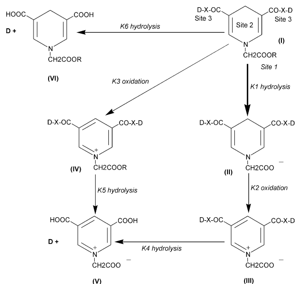
Scheme 1. Representative outline for the chemical delivery system design and work rationale; D = drug; X = NH, or O; R = alkyl.
