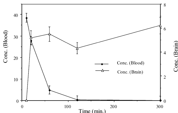
Figure 2. In vivo distribution of tryptamine-CDS ( 2a ) in blood and in rat brain homogenate (concd in µg/g against time in minutes).
